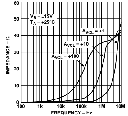
Closed-Loop Output Impedance vs. Frequency
