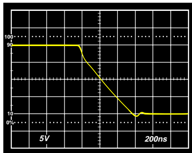
Negative Slew Rate R_L = 2\text{ k}\Omega , V_S = \pm 15\text{ V} , A_V = +1
