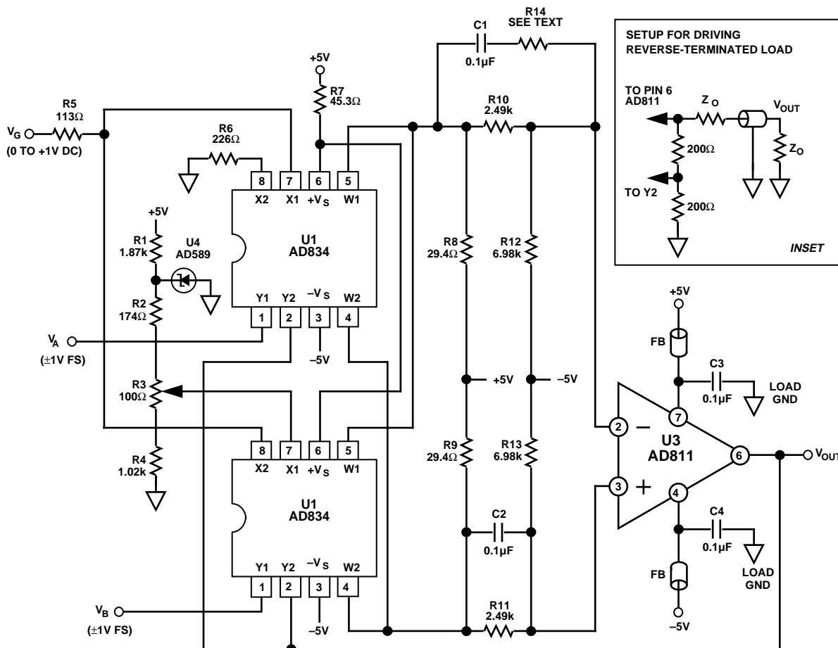
Figure 41. A Practical Video Keyer Circuit
