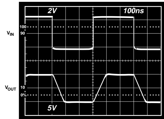
Figure 34. Output Waveform of an AD811 Driving a 500 pF Load. Gain = +2, R_{FB} = 649 \Omega , R_S = 15 \Omega , R_S = 10 \text{ k}\Omega
